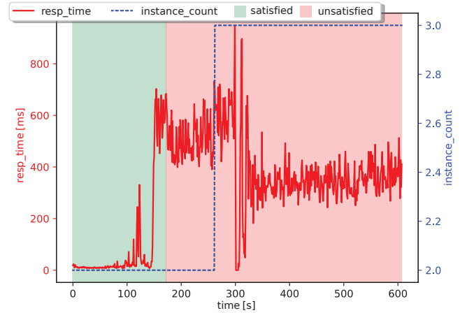
Figure 4: Result visualization for Chaos Experiment 2
