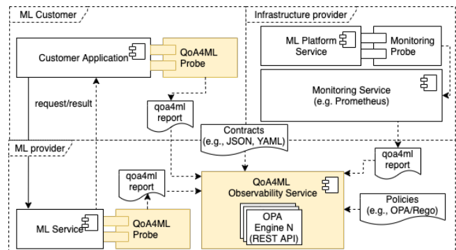
Figure 1: Integrating QoA4ML into an ML serving pipeline.
