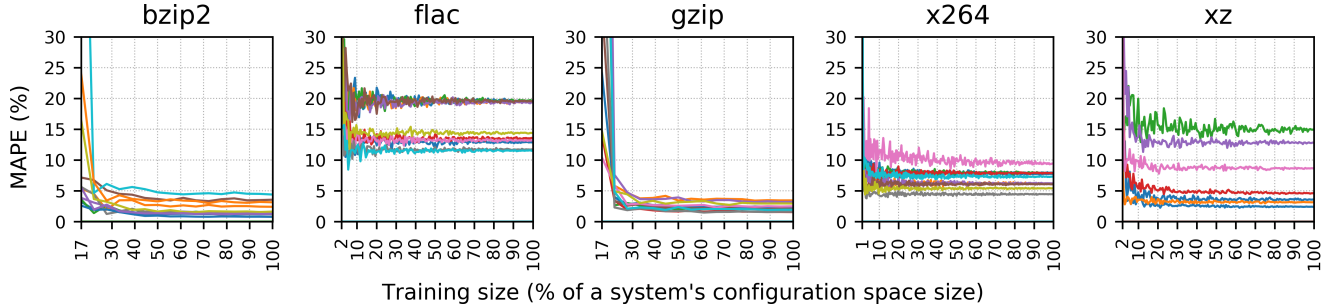
Figure 3: MAPE error distributions when transferring compression time metric using linear models as transferers. Each line represents the error's distribution on a particular hardware.
