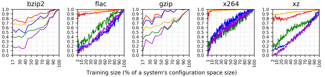
Figure 5: Classification measures' distributions, applied to evaluation of Pareto frontiers, approximated using regression trees. Each line represents a particular measure: TPR (green), TNR (red), PPV (blue), NPV (orange), MCC (violet).
