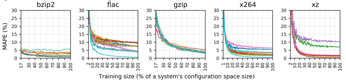
Figure 4: MAPE error distributions when transferring compression time metric using regression trees as transferers. Each line represents the error's distribution on a particular hardware.
