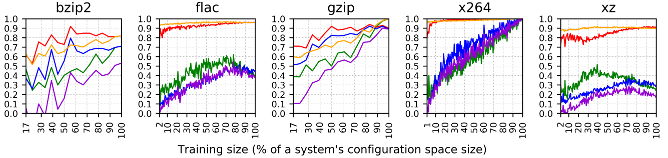
Figure 6: Classification measures' distributions, applied to evaluation of Pareto frontiers, transferred using linear models. Each line represents a particular measure: TPR (green), TNR (red), PPV (blue), NPV (orange), MCC (violet).
