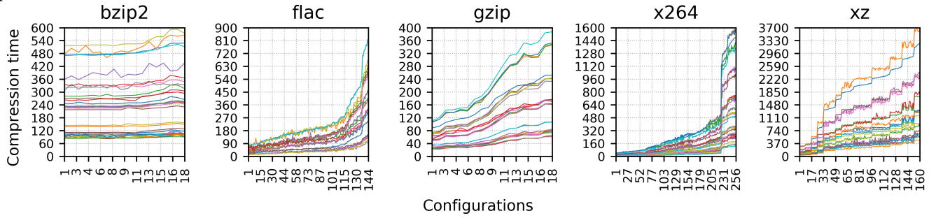
Figure 1: Compression time metric distributions for each software system. Each line represents the metric's distribution on a particular hardware.
