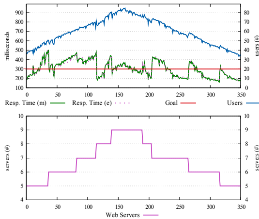
Figure 6: Behaviour of the system with a real deployment on Amazon EC2. Regular workload was used and the goal was set at 300 ms.
