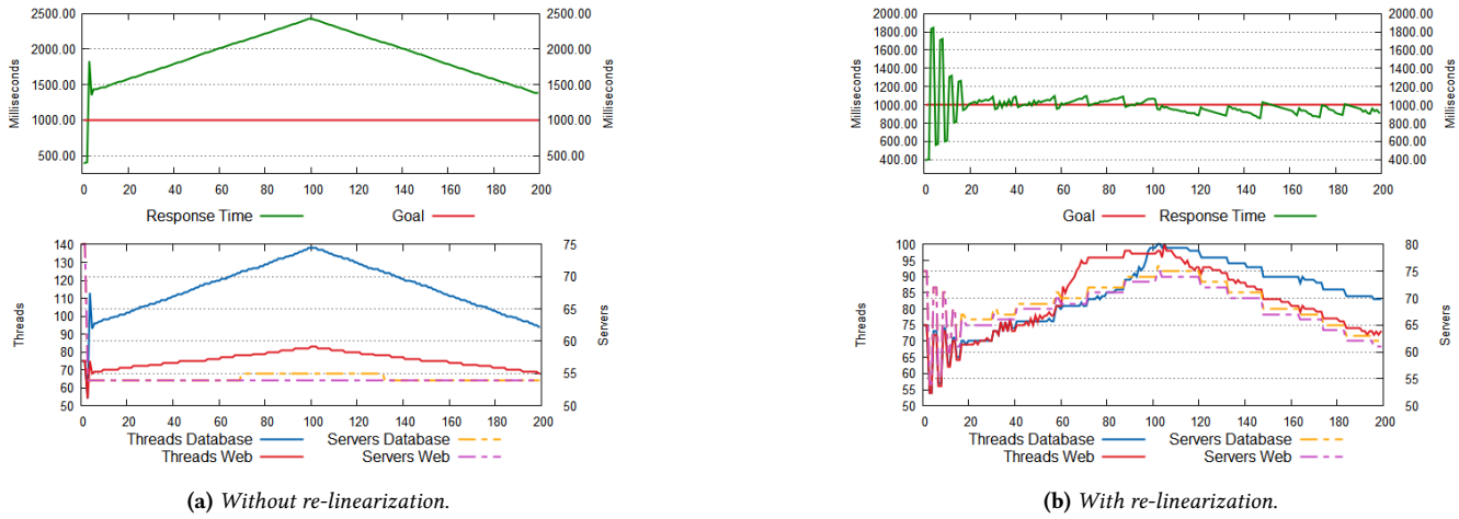
Figure 3: Behaviour of the system when the goal for Response Time was set to 1000 ms and the workload monotonically increases / decreases.
