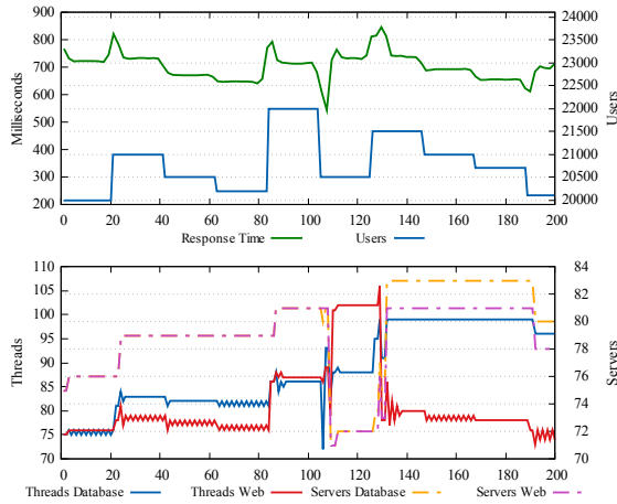
Figure 4: Behaviour of the system when the goal for Response Time was set to 700 ms, and the workload increasing/decreasing suddenly.
