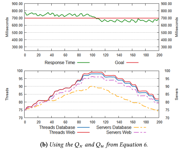
Figure 5: The effect of the weight matrices Q_x and Q_u on the behaviour of the controller.
