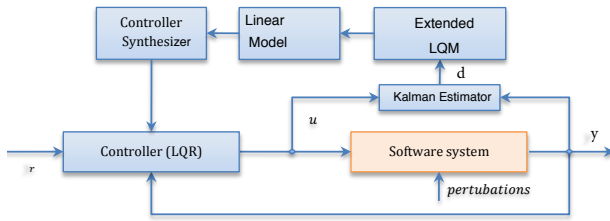
Figure 2: Model Identification Adaptive Control Architecture.
