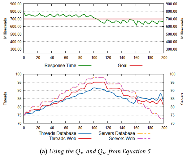
Figure 5: The effect of the weight matrices Q_x and Q_u on the behaviour of the controller.
