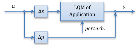
Figure 1: Extended LQM. Includes structural uncertainties
