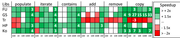
(c) HashSet primitive alternatives
