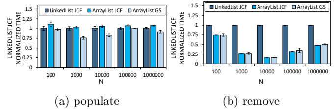
Figure 7: Execution time profiles of LinkedList for populate and remove scenarios.
