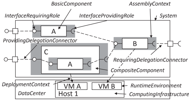
Figure 1: DML overview.
