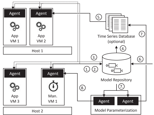
Figure 2: Reference architecture.
