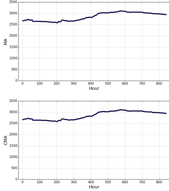
Figure 11: (a) Weekly moving average ( MA_t ) and (b) centered moving average ( CMA_t )
