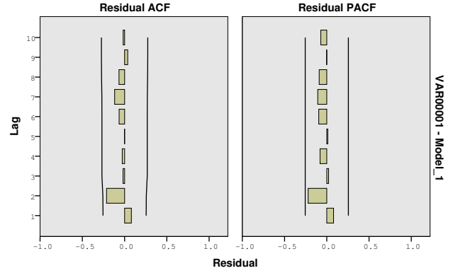
Figure 10: ACF and PACF of ARIMA(7,1,0)
