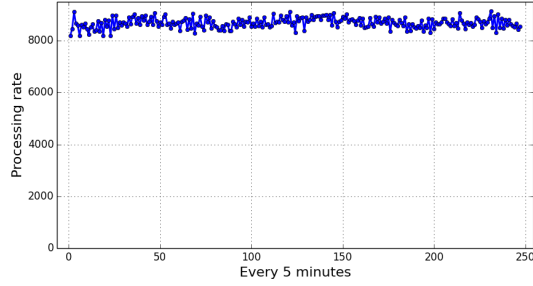
Figure 5: Relay processing rate (Relay capacity)
