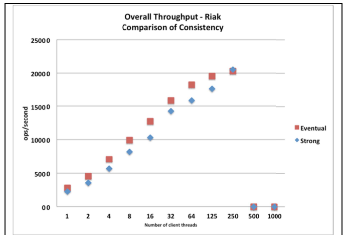
Figure 8 - Riak – Comparison of strong and eventual consistency
