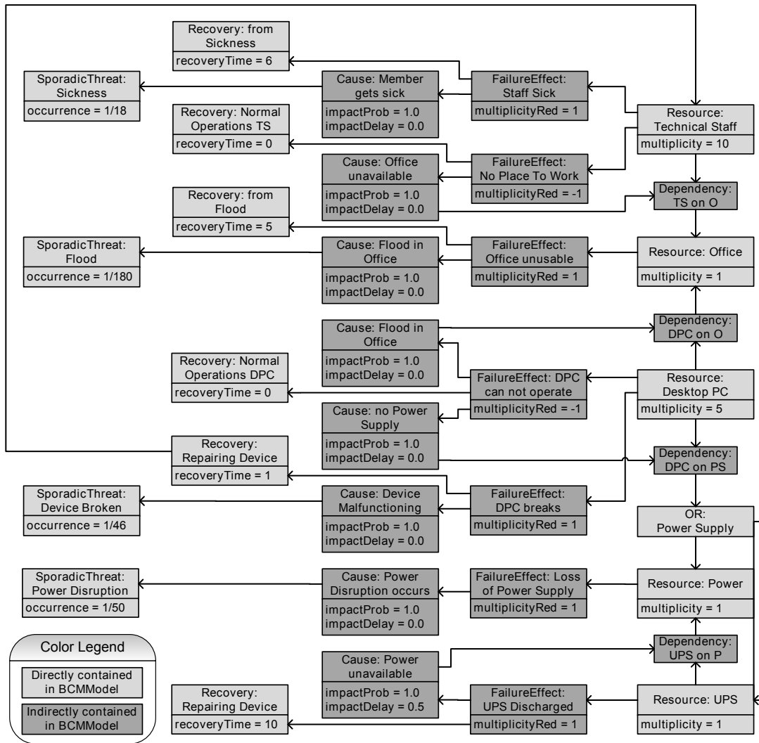
Figure 8: Complete GenericBCM model
