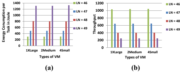
Figure 6. Energy Consumption (a) and Throughput (b).
