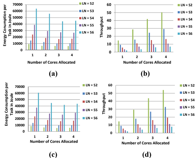
Figure 5. Energy Consumption (a) and Throughput (b) obtained by StressCloud; Energy Consumption (c) and Throughput (d) obtained manually.
