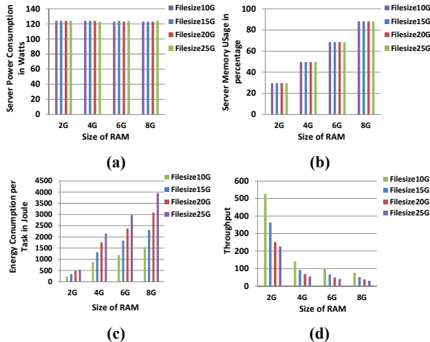
Figure 7. Server Power Consumption (a) and Memory Usage (b); Task Energy Consumption (c) and Throughput (d).
