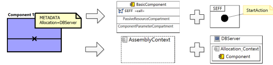
Figure 4: UCM2PCM Mappings - Standard Component
