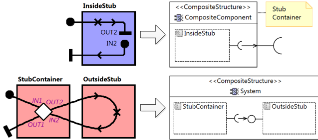
Figure 11: UCM2PCM Mappings - ParentCall
