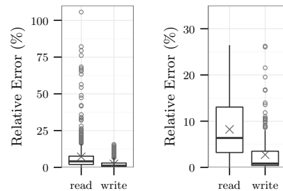
Figure 5: Prediction Accuracy of Queueing Models
