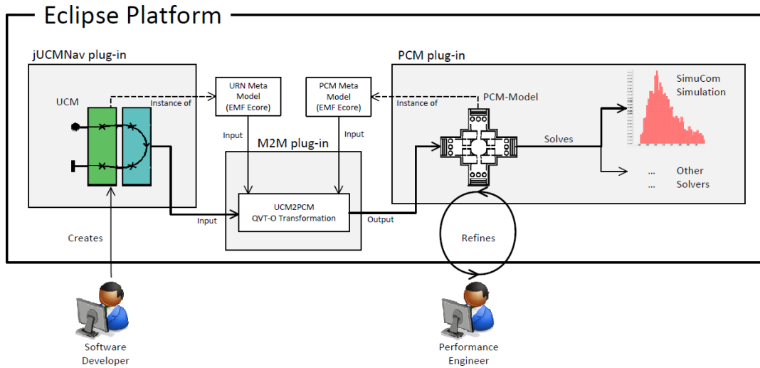
Figure 17: UCM2PCM Toolchain
