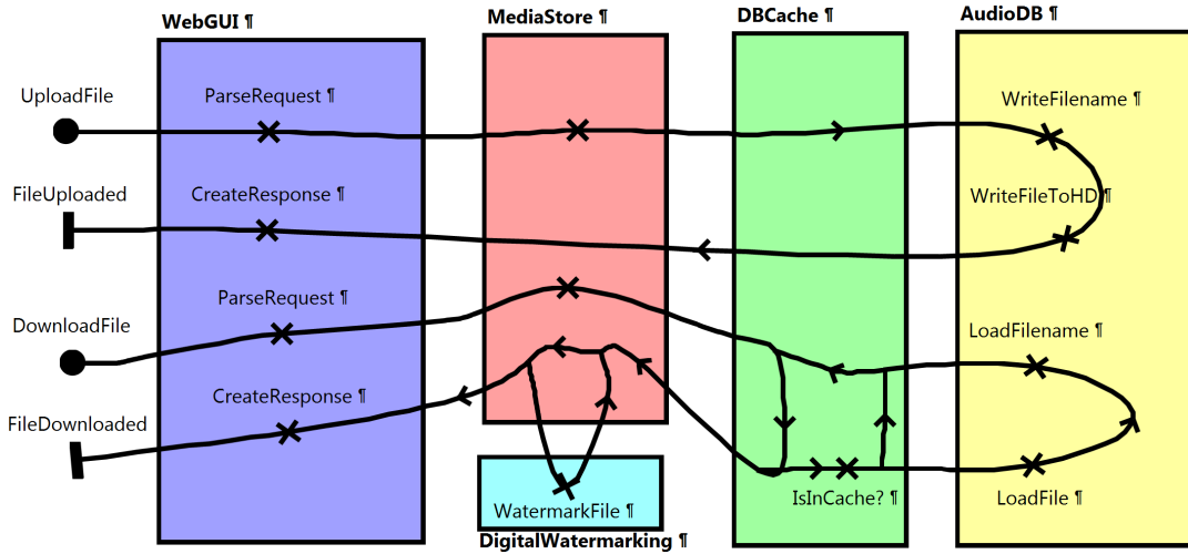
Figure 1: UCM of the Media Store components and inner control flow. The usage model is another UCM belonging to the model, which is omitted here for space reasons.
