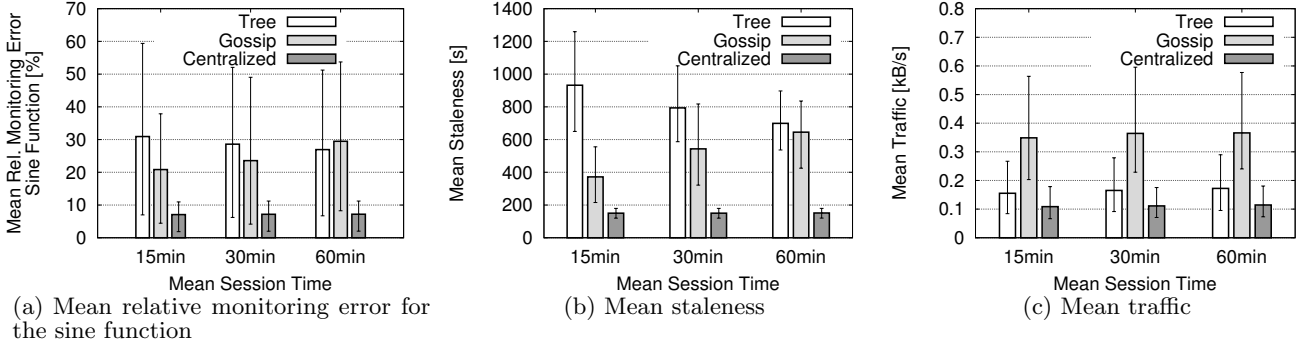
Figure 6: Per peer results for performance and costs, measured during the churn workload.
