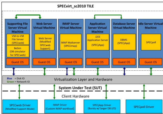
Figure 1. One Tile of SPECvirt_sc2010
