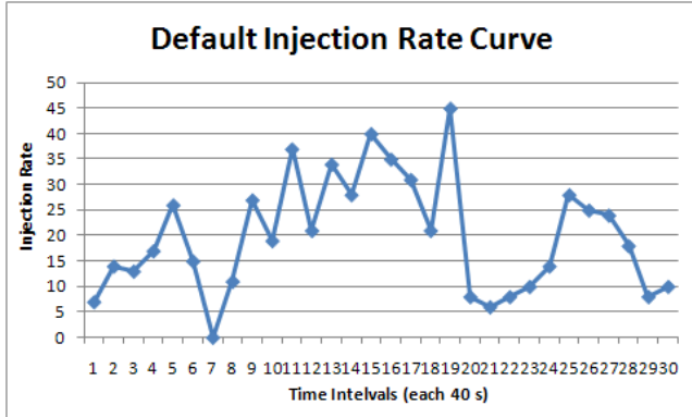
Figure 2. Default injection rate variation in SPECjAppServe2004*.
