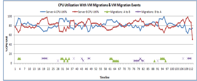
Figure 5. VM migrations and CPU utilization
