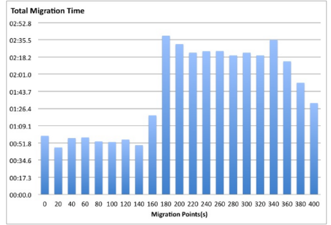
Figure 1: Total migration time results at different migration points
