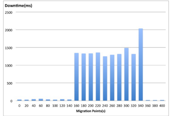
Figure 2: Downtime results at different migration points
