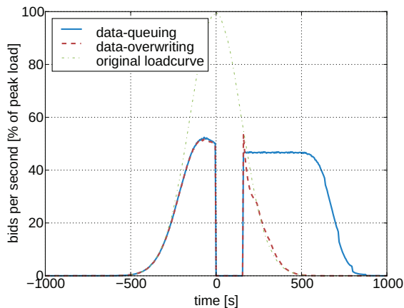
Figure 3: Transmission failure mitigation
