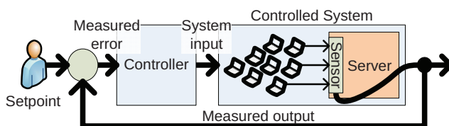
Figure 5: Control loop. Our controlled system consists of the individual clients and the server. A sensor at the server measures the processing delay. The measured error between an externally provided setpoint and the measured output is fed into the controller, which adjusts the system input accordingly. The system input is provided via a distributed feedback channel back to the clients.
